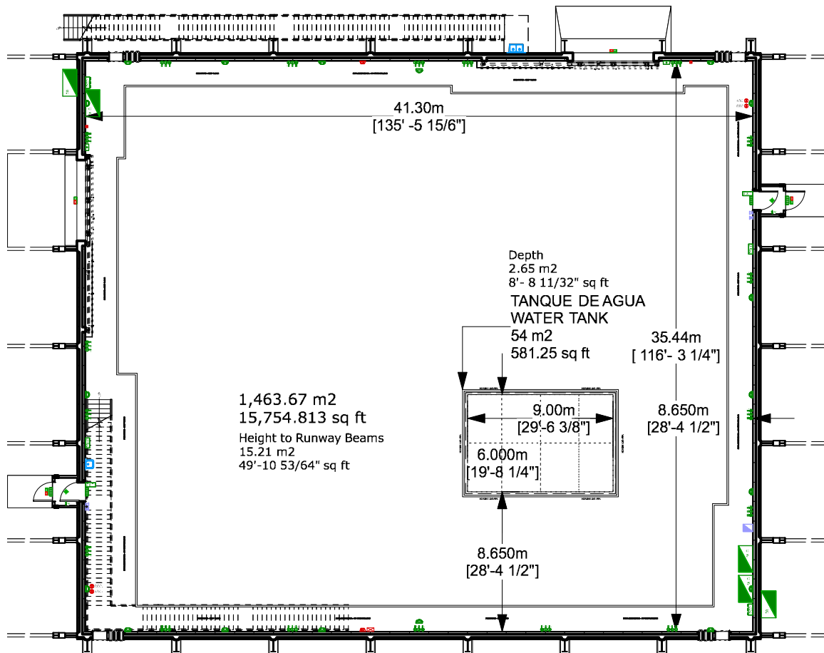
SS2 GROUND FLOOR Scale: 1:333
